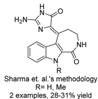
Scheme 23 General transformation of oxazolone to imidazolone.
