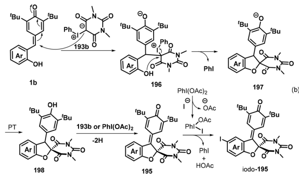
Scheme 55 [4 + 1] annulation of p -QMs with iodonium ylides.
