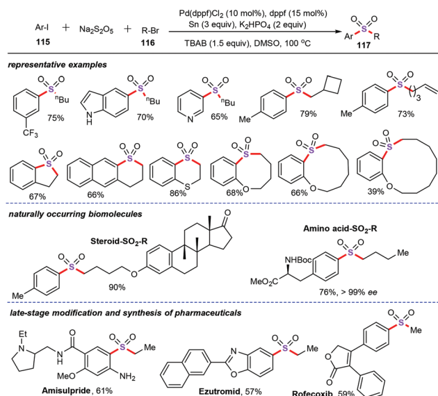
Scheme 44 Palladium-catalyzed multicompound reductive cross-coupling reaction.
