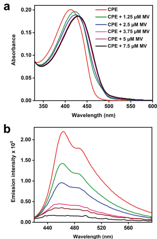
Fig. 2 (a) Absorption and (b) fluorescence spectra ( \lambda_{ex} = 410 nm) of CPE (5 μM, PRU) in water with varying concentrations of MV 2+ as indicated in the figure.
