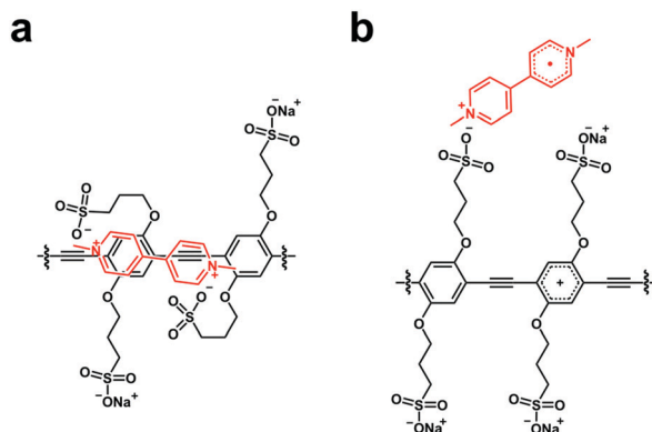
Fig. 7 Possible structure of ion-pair complexes. (a) [CPE, MV^{2+} ] and (b) [CPE ^{\bullet+} , MV^{\bullet+} ].
