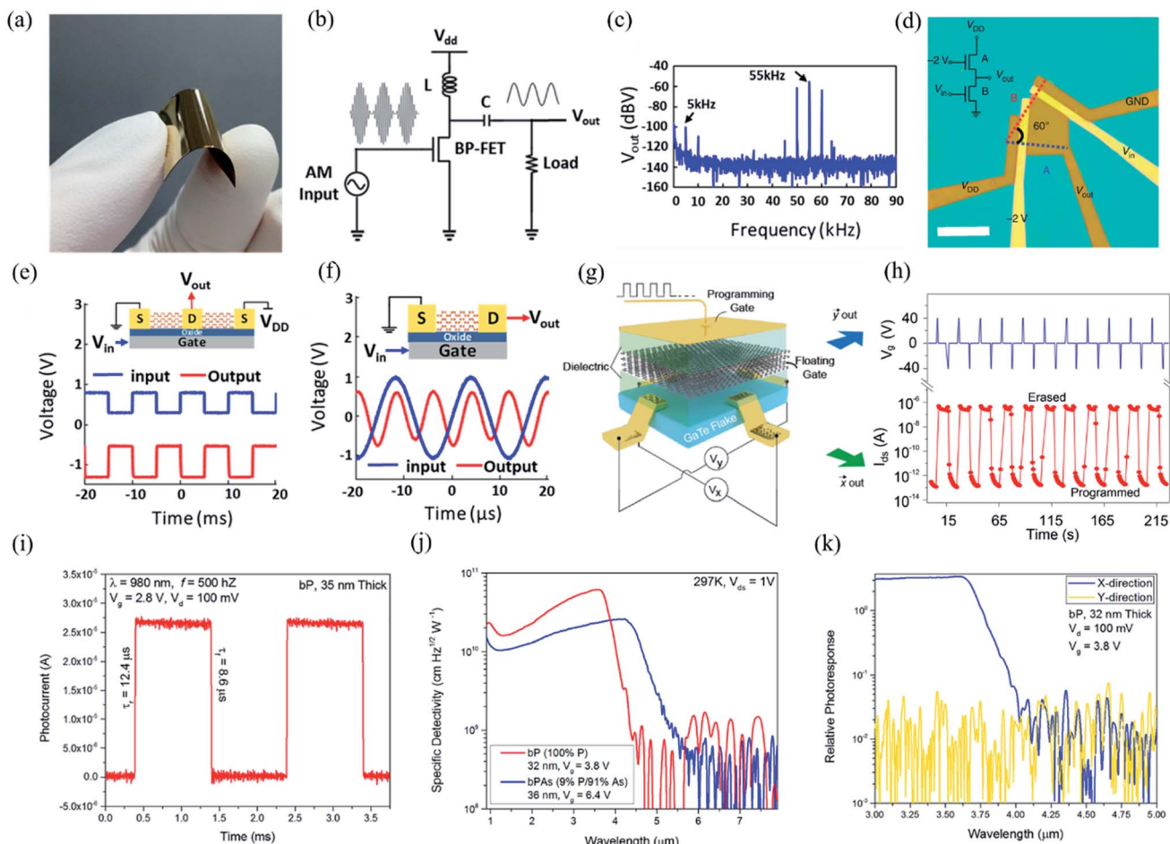
Fig. 17 (a) Optical image of few-layer BP devices on a flexible substrate. (b) Schematic of an ideal AM demodulator system based on BP FET operating at the ambipolar point. (c) Output spectrum of the ambipolar transistor demodulator showing the demodulated baseband signal (5 kHz) and the modulated carrier feed-through (55 kHz). Input carrier V_{pp} = 100 mV. Reproduced from ref. 214 with permission from American Chemical Society. (d) Optical image of a typical inverter device based on few-layer \text{ReS}_2 flake. The scale bar is 10 \mu\text{m} . The inset is the circuit diagram of the inverter, where the top-gate voltage along the a -axis is fixed at 2 V, the top-gate voltage along the b -axis is the input voltage V_{in} , and the middle shared electrode is the output voltage V_{out} . Reproduced from ref. 35 with permission from Nature Publishing Group. (e) The ambipolar digital inverter based on BP at V_g = -0.46 V and V_{dd} = -2 V. Input pulse oscillates at 100 Hz with peak-to-peak amplitude ( V_{pp} ) of 0.5 V. Inverter output pulse showing a gain of about 1.6. (f) Ambipolar single FET frequency doubler based on BP at V_g = 0 V and V_d = -1 V. Input signal is 64 kHz sinusoid with V_{pp} = 2 V. Output signal oscillates at the double frequency (128 kHz) with a voltage gain of about 0.7. Reproduced from ref. 214 with permission from American Chemical Society. (g) The schematic view of a typical anisotropic memristor based on h-BN/GaTe/h-BN heterojunction with a graphite floating gate. (h) Demonstration of erasing and programming pulses measured in the y -direction. Reproduced from ref. 36 with permission from Nature Publishing Group. (i) Room-temperature temporal photoresponse of a 35 nm-thick BP photoconductor, excited by a 980 nm laser modulated at 50 kHz. ( \lambda = 980 nm, f = 500 Hz, V_g = 2.8 V, V_d = 100 mV, t_r = 12.4 \mu\text{s} , \text{set } 98 = 1 ). (j) Specific detectivity of BP and b-PAs photoconductors with optimized thickness and gate voltage at room temperature. 217 (k) Relative response of a BP photoconductor measured for incident light polarized along the x (armchair) and y (zigzag) directions of the BP crystal. Reproduced from ref. 217 with permission from American Chemical Society.
