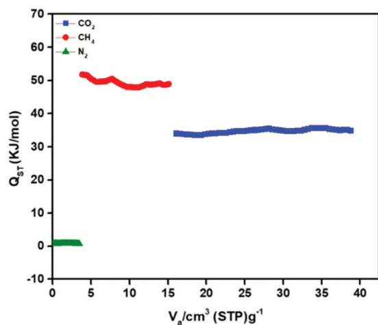
Fig. 5 Isotheric heat of adsorption ( Q_{st} ) for CO 2 , CH 4 and N 2 using experimental isotherm data of Zn-CBS at 263 K, 273 K and 298 K.
