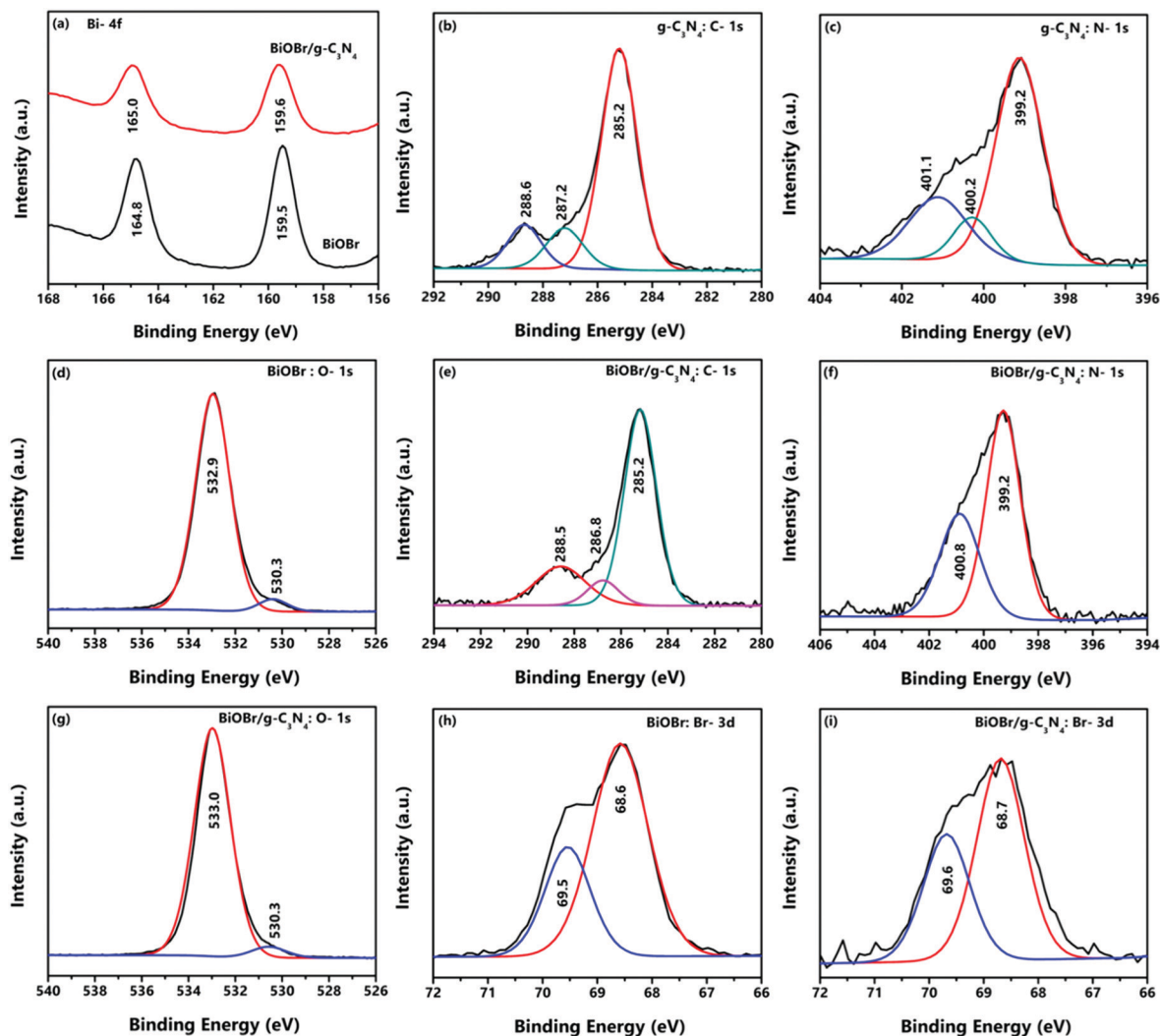
Fig. 7 High resolution XPS spectra of g\text{-C}_3\text{N}_4 , BiOX and the BiOX/ g\text{-C}_3\text{N}_4 composite.
