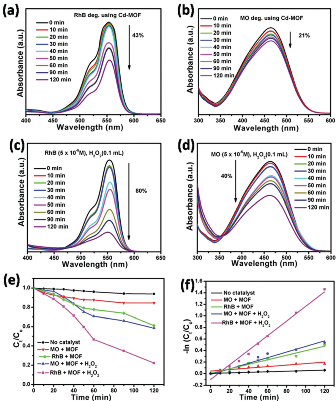
Fig. 18 UV-vis spectra for the photocatalytic degradation of RhB and MO (a) and (b) over Cd-MOF and (c) and (d) with the addition of H_2O_2 . Kinetic plots for the photocatalytic degradation of RhB and MO under various parameters (e) and (f). Reproduced from ref. 269 with permission from the Royal Society of Chemistry.
