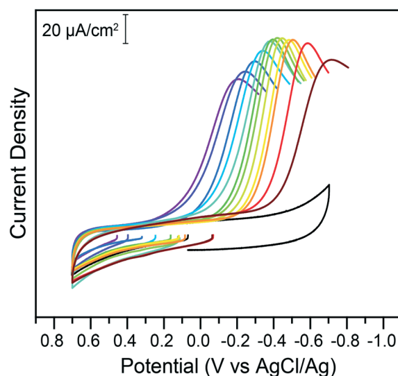
Fig. 4 Cyclic voltammograms of 200 \mu M potassium chromate in 1 M KCl electrolyte in the absence (black) or presence of 0.1 M citric acid buffer at various pH values, on glassy carbon electrodes. All data was collected at 100 mV s^{-1} . The pH of the buffer, from the purple to the brown trace, is 2.25, 2.5, 3.0, 3.25, 4.0, 4.5, 5.0, 5.25, 5.50, 6.0, 6.25, and 6.75. Return traces not shown for clarity. Full traces available in the ESI†
