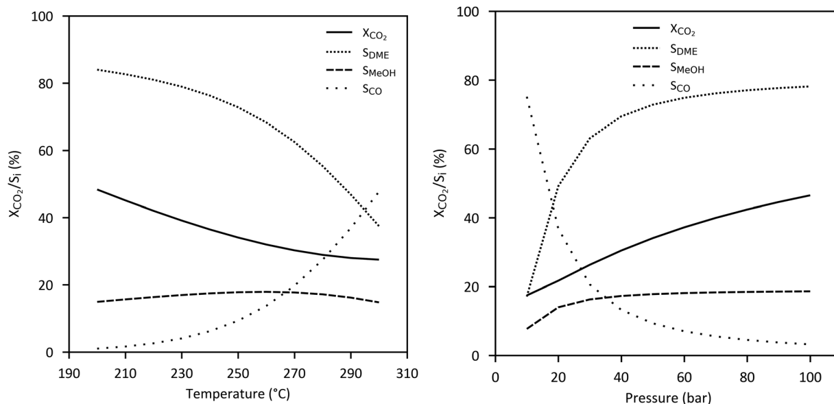
Fig. 13 Equilibrium conversion of CO 2 ( = [CO_{2,in} - CO_{2,out}]/CO_{2,in} ) and selectivity of DME, methanol and CO ( S_i = i/[CO_{2,in} - CO_{2,out}] , with i = 2 \times DME/MeOH/CO , based on amount of C-atoms) dependent on (a) temperature and (b) pressure ( H_2 : CO_2 = 3 : 1 , based on Aspen Plus Simulation).
