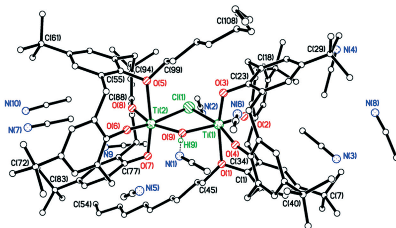
Fig. 7 Molecular structure of \{[\text{Ti}(\text{L})(\text{O})_3(\text{On-decyl})_2]_2(\mu\text{-Cl})(\mu\text{-OH})\} \cdot 8.5\text{MeCN} (10·8.5MeCN) (most H atoms are omitted for clarity). Selected bond lengths (Å) and angles ( ^\circ ): Ti(1)–O(1) 2.381(3), Ti(1)–O(2) 1.817(3), Ti(1)–O(3) 1.852(3), Ti(1)–O(4) 1.793(3), Ti(1)–O(9) 2.000(3), Ti(1)–Cl(1) 2.5177(14); O(1)–Ti(1)–O(3) 168.54(13), O(2)–Ti(1)–O(4) 102.84(15), Cl(1)–Ti(1)–O(9) 74.82(10), Ti(1)–O(1)–C(1) 112.8(2), Ti(1)–O(2)–C(12) 150.5(3), Ti(1)–O(3)–C(23) 119.9(2), Ti(1)–O(4)–C(34) 168.3(3).
