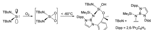
Scheme 35 Synthesis of the silanol 90 .
