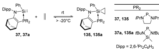
Scheme 54 Reversible addition of ethylene to the phosphine silylene complexes 37 and 37a .
