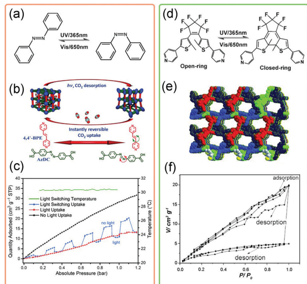
Fig. 22 (a) Scheme of the conformational changes of the azobenzene molecule upon UV irradiation. (b) Illustration of the guest triggered framework changes of Zn(AzDC)(4,4'-BPE) 0.5 . (c) CO 2 adsorption isotherms of Zn(AzDC)(4,4'-BPE) 0.5 at 303 K in the presence of light (red), absence of light (black) and light switching environment (blue). (d) Scheme of the conformational changes of the diarylethene molecule upon UV irradiation. (e) Crystal structure of the diarylethene MOF. (f) The static and dynamic CO 2 isotherms under different conditions. Partly taken from ref. 134 and 138 with permission.
