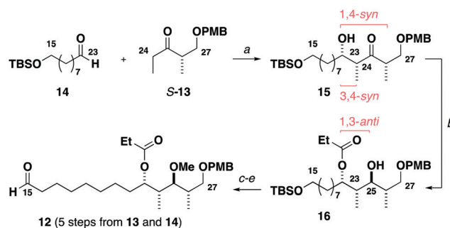
Scheme 2 Synthesis of the C15–C27 aldehyde 12. Reagents and conditions: (a) S -13, Ti(OiPr) 3 , DIPEA, CH 2 Cl 2 , –78 °C; 14, CH 2 Cl 2 , –78 °C, 85%, 18:1 dr, (b) SmI 2 , EtCHO, THF, –20 °C, 95%, >20:1 dr, (c) Me 3 O-BF 4 , Proton Sponge®, CH 2 Cl 2 , r.t., 89%, 99% brsm, (d) HCl (3 M)/THF/H 2 O (5:2:1), r.t., 99%, (e) (COCl) 2 , DMSO, CH 2 Cl 2 , –78 °C; Et 3 N, –78 °C to r.t., 94%.
