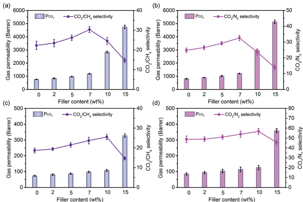
Fig. 3 The effect of the COF-300 filler content on membrane separation performance tested at 25 °C with a transmembrane pressure of 1 bar. (a) CO_2/CH_4 and (b) CO_2/N_2 separation performance of COF-300/6FDA-DAM series MMMs. (c) CO_2/CH_4 and (d) CO_2/N_2 separation performance of COF-300/Pebax series MMMs.
