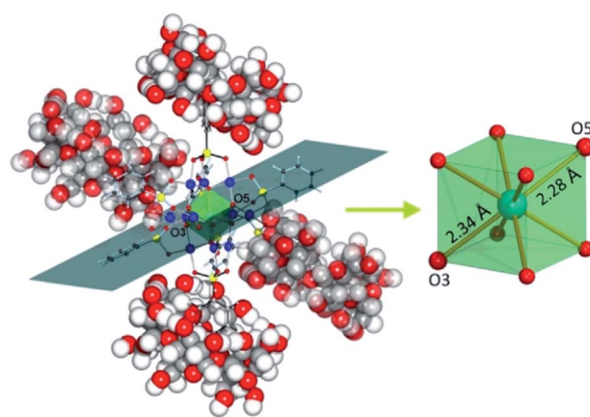
Fig. 11 Representation of the fragment of the solid-state structure of K_6\{[CoO_8Pd_{12}(C_6H_5AsO_3)_8]\} \cdot 2\{C_{36}H_{60}O_{30}\} \cdot 25H_2O \cdot KCl , emphasizing the elongation of the \{CoO_8\} unit (transparent green) along one of its diagonal planes. Bonds in the two \alpha -CD-incorporated phenyl-arsonates are shown in black. Counterions, water and co-crystallised KCl molecules are omitted for clarity. Color code: Co, turquoise; Pd, blue; As, yellow; O, red; C, black/grey; H, white spheres. Reprinted with permission from ref. 74c. Copyright 2018 of Wiley-VCH Verlag GmbH & Co. KGaA.
