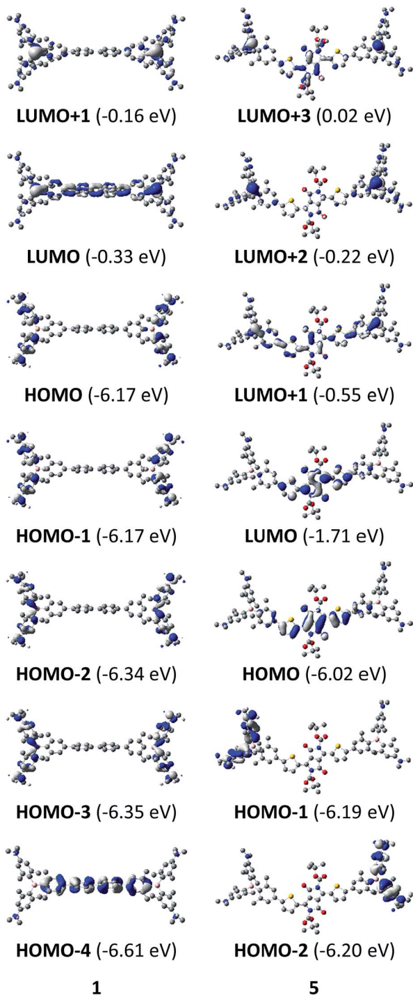
Fig. 2 DFT (CAM-B3LYP/6-31G(d))-calculated relevant orbitals for 1 and 5 . Hydrogen atoms are omitted for clarity. Surface isovalue: \pm 0.03 [ e_0^{-3/2} ]. Orbital energy differences are not direct approximations of excitation energies. They are provided here for comparison between the compounds.
