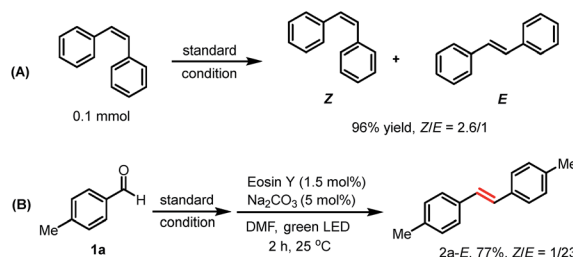
Scheme 4 Isomerization studies.
