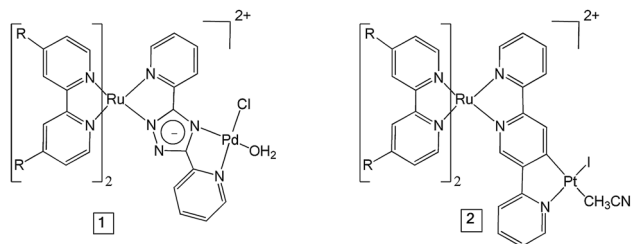
Fig. 1 The structures of the dye-catalyst assemblies 1 and 2 (R = CO 2 Et).
