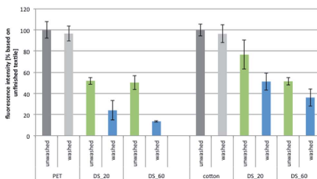
Fig. 6 Results of the protein adhesion tests for PVAm-g-PEGMA on PET and cotton. The fabrics were finished with different degrees of substitution (DS) and then used either directly after rinsing with water (unwashed) or after 5 wash cycles according to DIN EN ISO 105-C06 using ECE detergent (washed).
