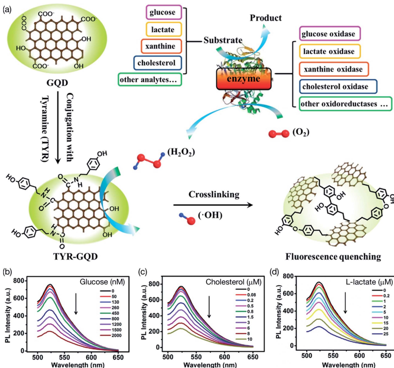
Fig. 32 (a) Schematic illustration of fluorescence detection scheme using tyramine-functionalized GQDs (TYR-GQDs). (b) Photoluminescence (PL) spectra of 0.1 mg \text{mL}^{-1} TYR-GQD in PBS (pH 7.0) containing 2.5 \mu\text{M} glucose oxidase and at different concentrations of glucose. (c) PL spectra of spectra of 0.1 mg \text{mL}^{-1} TYR-GQD in PBS (pH 7.0) containing 10 \mu\text{M} cholesterol oxidase and at different concentrations of cholesterol. (d) PL spectra of 0.1 mg \text{mL}^{-1} TYR-GQD in PBS (pH 7.0) containing 5 \mu\text{M} lactate oxidase and at different concentrations of L-lactate. [Reprinted with permission from ref. 670, N. Li, A. Than, X. Wang, S. Xu, L. Sun, H. Duan, C. Xu and P. Chen, Ultrasensitive Profiling of Metabolites Using Tyramine-Functionalized Graphene Quantum Dots, ACS Nano , 2016, 10, 3622–3629. Copyright© American Chemical Society.]
