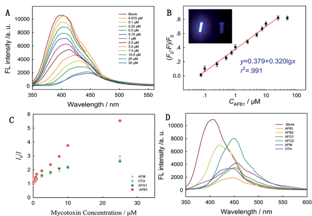
Fig. 3 Emission spectra of Zr-CAU-24 with the incremental addition of AFB1 in water, with toxin concentrations given from 0 to 50 μM (A). Linear relationship between \lg C_{\text{AFB1}} and FL intensity. Inset: optical photo of fluorescent Zr-CAU-24 crystals in water (left) and water (right) (B). Stern–Volmer curves acquired at \lambda_{\text{ex}} = 340 nm and \lambda_{\text{em}} = 410 nm for AFB1, AFG1, AFM and OTA (C). FL intensity fading of Zr-CAU-24 towards 50 μM AFB1, AFB2, AFG1, AFG2, AFM and OTA (D).
