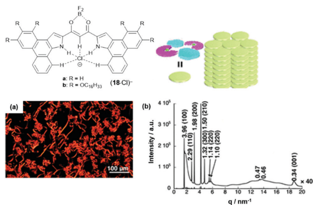
Fig. 18 Schematic representation of the phenanthro[ b ]-fused \pi -electronic anion ( 18\text{-Cl}^- ). (a) POM image of ( 14\text{a} )( 18\text{b-Cl}^- ) at 180\text{ }^\circ\text{C} upon cooling. (b) Synchrotron XRD pattern of ( 14\text{a} )( 18\text{b-Cl}^- ) at 150\text{ }^\circ\text{C} upon cooling; the proposed supramolecular packing mode of the assembly is also shown. 56 Figure reproduced with kind permission; © 2019 American Chemical Society.
