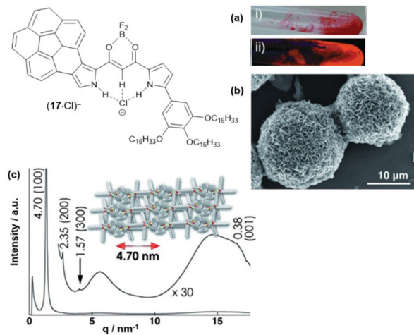
Fig. 17 Schematic representation of the \pi -electronic anion ( 17\text{-Cl}^- ). (a) Photographs of ( 14\text{a} )( 17\text{-Cl}^- ) in 1,4-dioxane under visible (i) and UV light (ii). (b) SEM image of the precipitated ( 14\text{a} )( 17\text{-Cl}^- ). (c) XRD pattern of ( 14\text{a} )( 17\text{-Cl}^- ) at 80\text{ }^\circ\text{C} on cooling from the Iso phase; the proposed supramolecular structure of the assembly is also shown. 55 Figure reproduced with kind permission; © 2013 Wiley-VCH.
