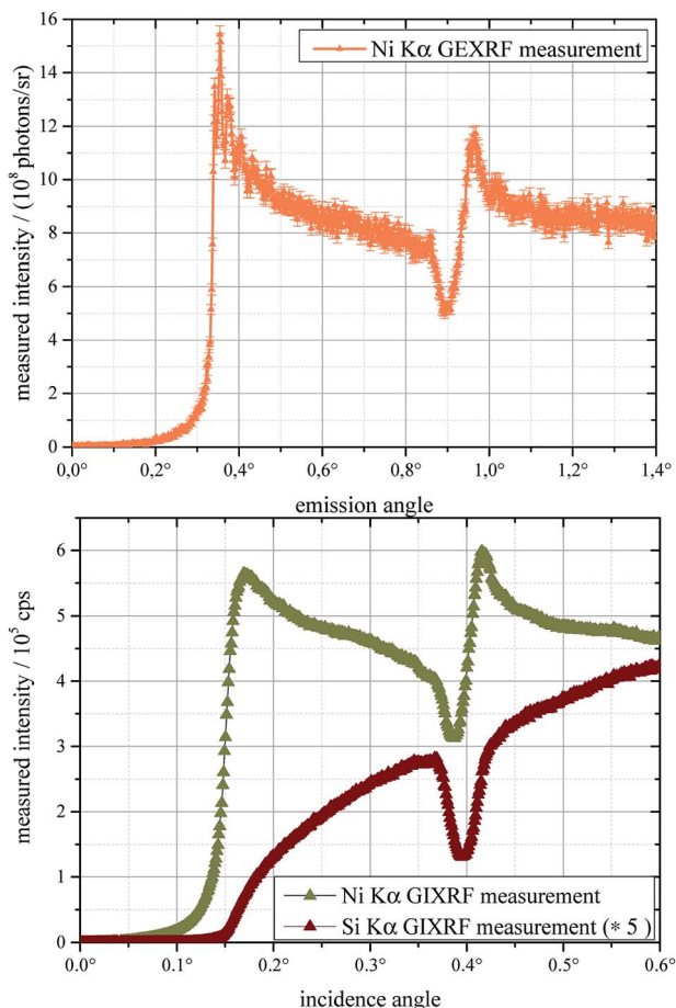
Fig. 4 Angle resolved elemental profiles of the NiC multilayer. For the SF-GEXRF measurements (top) only the Ni \text{K}\alpha fluorescence line profile is shown. An angular resolution of 0.005^\circ enables the discrimination of fine interference structures not visible in the respective GIXRF profile (bottom). The GIXRF profiles of the Ni \text{K}\alpha (green) and Si \text{K}\alpha (red) fluorescence lines are shown. The profile of silicon is multiplied by a factor 5 to display it in one plot with nickel.
