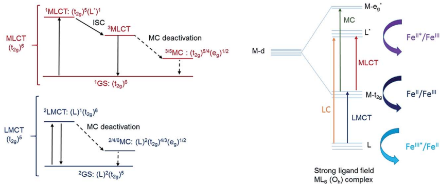
Fig. 2 Simplified Jablonski-type diagram for low-spin Fe^{II} 3d^5 and Fe^{III} 3d^6 complexes (left), together with a schematic illustration of key electronic levels and photoexcitation processes involved in the photophysics (right). Curved arrows indicate opportunities to drive subsequent bimolecular or interfacial electron transfer processes (far right).
