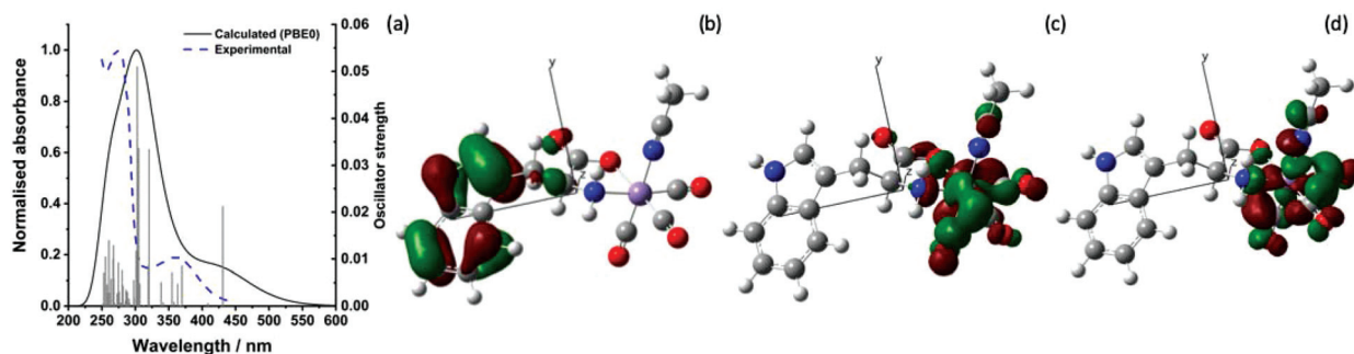
Fig. 2 (a) Experimental and predicted electronic spectra of trypto-CORM (b) HOMO 98 (c) LUMO 99 and (d) LUMO+ 100 calculated at the PBE0/DGDZVP/def2tzv level. Isosurface shown at the 0.04 level.
