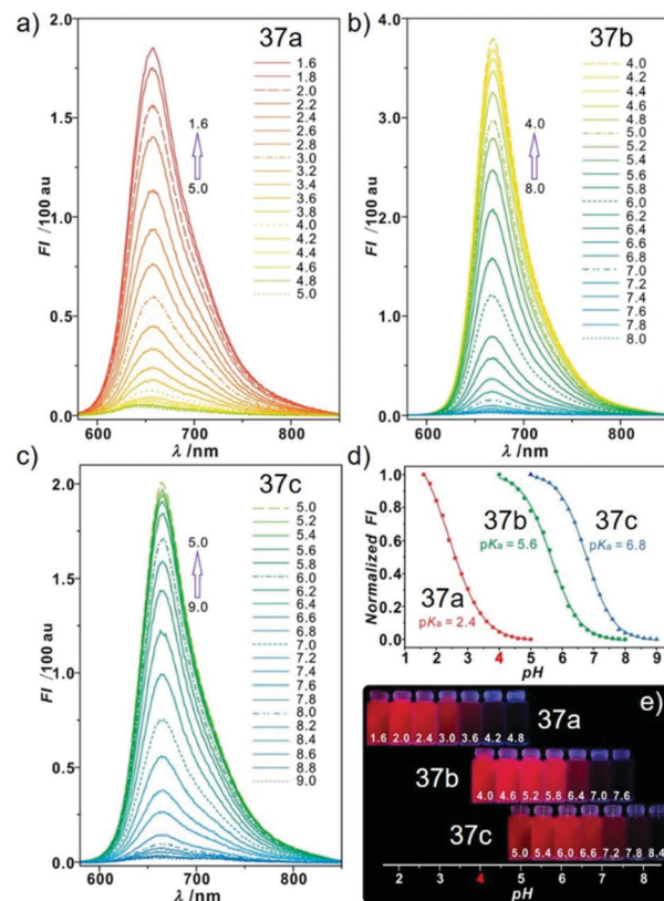
Fig. 56 pH activable emission properties of probes 37a–c (10 \mu\text{M} , \lambda_{\text{ex}} = 570 \text{ nm} ) in disodium hydrogen phosphate–citric acid buffers containing 10% DMSO: (a) probe 37a ; (b) probe 37b ; (c) probe 37c ; (d) normalized fluorescence intensities of probes 37a–c at different pH values at (a) 657 nm, (b) 668 nm, and (c) 663 nm; (e) photograph of pH-dependent red emissions under a 365 nm lamp in a darkroom. Copyright 2015 American Chemical Society.
