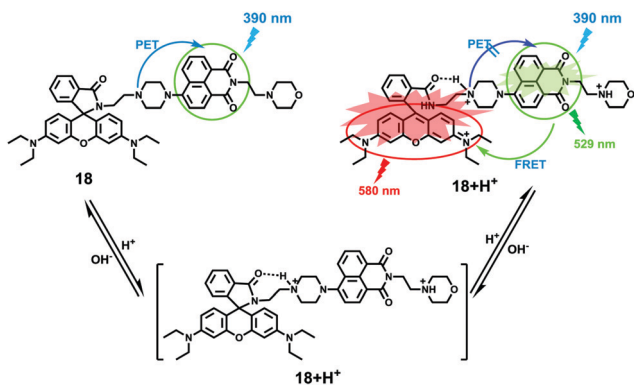
Scheme 13 Fluorescent probe 18 for pH.
