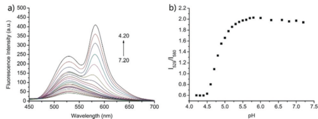
Fig. 23 (a) Fluorescence spectra of probe 18 (5 \mu\text{M} ) in the B-R buffer/EtOH (9/1, v/v) solution at different pH values (7.20, 7.00, 6.80, 6.60, 6.30, 6.00, 5.80, 5.70, 5.60, 5.50, 5.40, 5.30, 5.20, 5.10, 5.00, 4.90, 4.80, 4.70, 4.60, 4.50, 4.40, 4.30, and 4.20); and (b) the plot of the emission ratios of R at I_{529}/I_{580} versus pH values; \lambda_{\text{ex}} = 390 nm. Copyright 2015 Royal Society of Chemistry.
