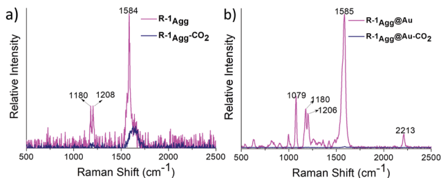
Fig. 4 (a) Raman spectra of R-1 Agg ( 4 \times 10^{-4} M) in aqueous medium (water/THF, 99/1 v/v) and after purging with CO 2 . (b) SERS spectra of R-1 Agg in the presence of Au-NPs (1/9 v/v) and after purging with CO 2 .
