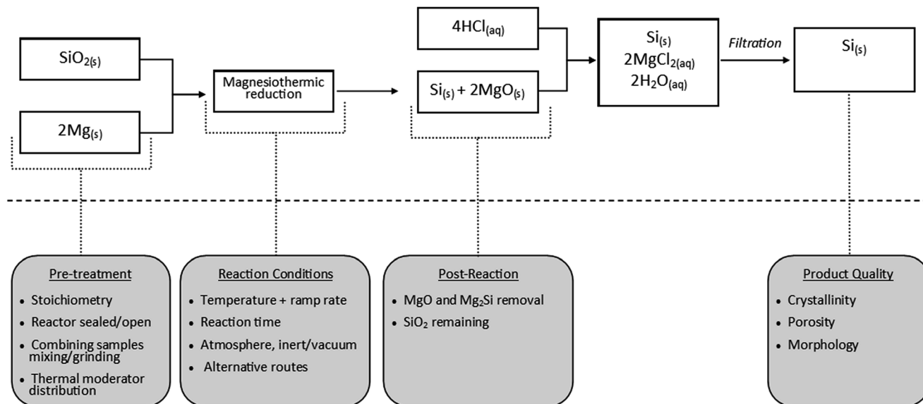
Fig. 6 Scheme outlaying the magnesiothermic reduction and summary of key design factors for consideration.
