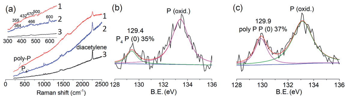
Fig. 4 (a) Raman spectra of the MOF (curve 1), MOFs@ P_4 (curve 2) and irradiated MOFs@ P_4 (curve 3), respectively; (b) XPS spectrum of the P 2p envelope of MOFs@ P_4 ; (c) XPS spectrum of the P 2p envelope of irradiated MOFs@ P_4 .
