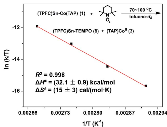
Fig. 9 Eyring plot of the reaction of 1 with TEMPO. Conditions: 1.6 \text{ mmol L}^{-1} of 1 , 16 \text{ mmol L}^{-1} of TEMPO, toluene- d_8 (containing 15% v/v \text{C}_6\text{D}_6 ), in the dark and under a \text{N}_2 atmosphere.
