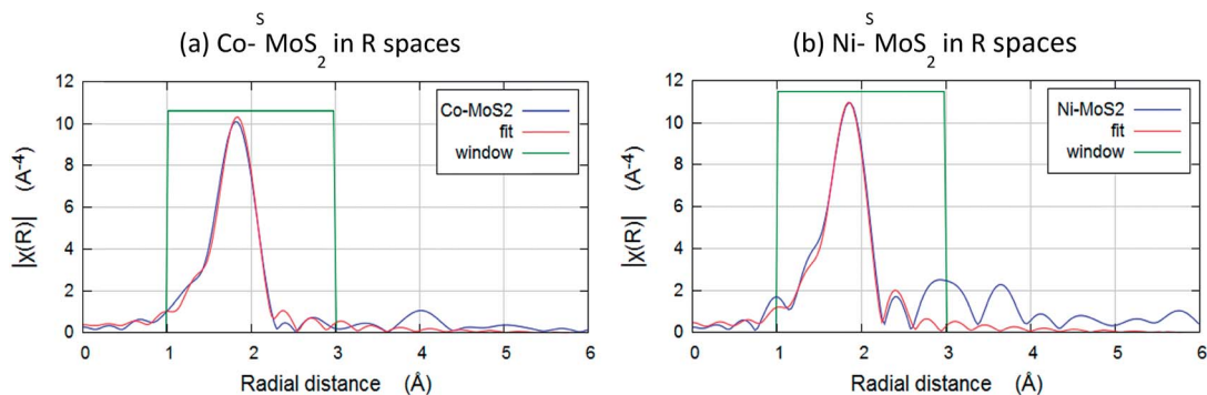
Fig. 6 Fourier transforms of the k^3 -weighted Co and Ni K-edge of extended X-ray absorption fine structure spectroscopy (EXAFS) spectra of (a) \text{Co-MoS}_2 and (b) \text{Ni-MoS}_2 .
