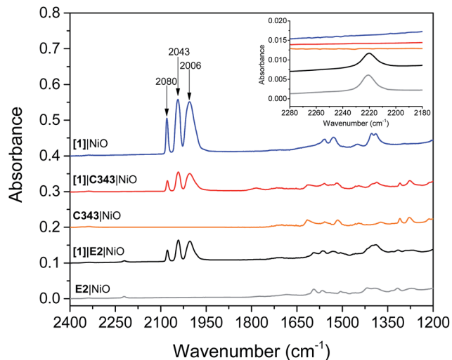
Fig. 2 FTIR absorption spectra of the co-sensitized NiO films, [1]|E2|NiO (black) and [1]|C343|NiO (red). The reference sensitized films, [1]|NiO (blue), E2|NiO (gray), C343|NiO films (orange), are also shown. The spectra have been offset by 0.1 absorbance units. Inset in panel B shows the region of the \nu_{\text{C}\equiv\text{N}} stretch of the E2 dye.
