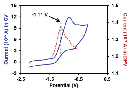
Fig. 2 CV and DPV plots of 2 mM complex 4 ·DME in THF (0.1 M n-Bu_4N^+PF_6^- as the supporting electrolyte). The blue solid line: CV plot (scan rate = 0.1\text{ V s}^{-1} ); the red dashed line: DPV plot.
