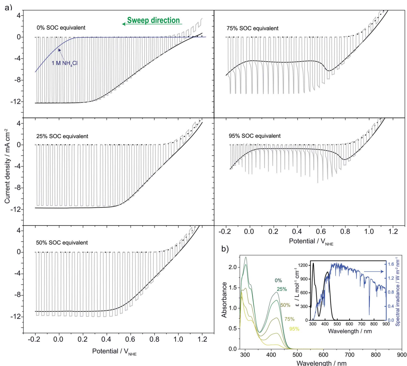
Fig. 5 (a) LSVs recorded on \text{pn}^+\text{Si}/\text{TiO}_2 in 0.4 M ferro/ferricyanide solutions in ratios matching that expected for different SOC equivalents in the solar flow battery (SOC equivalents) and of the pure supporting electrolyte (1 M \text{NH}_4\text{Cl} displayed with the 0% SOC equivalent, blue line) relative to a reference electrode. Recorded in constant light (1 sun, full black line), chopped (full grey line) and dark (dotted black line behind chopped). (b) The measured absorbance of the SOC equivalent solutions (diluted 300 times) and the inset shows the calculated associated extinction coefficient (black) overlaid on the AM1.5G spectrum (blue) (see S7 † ). 27
