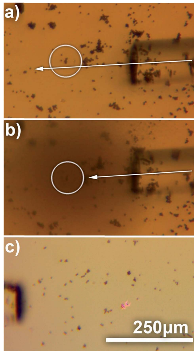
Fig. 4 Optical microscopy image demonstrating importance of alignment between the plasmon-magnetic material and the laser beam. In (a) small clump of Au nanocages-covered microbeads (~10 beads) is slightly misaligned with the laser beam, and even though the laser is on, no heat is generated. In (b) optical fiber is aligned to the clump and the area inside of the white circle is heated on average above 34 °C (see the image luminosity analysis in ESI† for details). (c) Shows control experiment when the microbeads are not decorated with Au nanocages. IR filter is removed to demonstrate direct exposure of the micro-beads to the laser light. No heating is observed.
