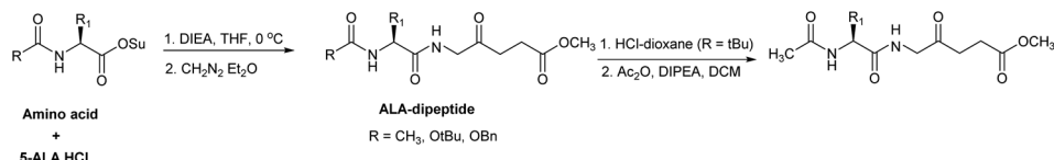
Scheme 10 Synthesis of ALA peptide derivatives by Rogers et al. avoiding self-condensation of ALA during the coupling step.
