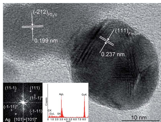
Fig. 27 HRTEM image of Ag 2 S/Ag heterostructures. Monoclinic (space group P2_1/c ) Ag 2 S nanoparticle with an \alpha -Ag 2 S acanthite structure (upper left corner) is in direct contact with a cubic (space group Fm\bar{3}m ) Ag nanoparticle. The electron diffraction pattern obtained by FFT of the HRTEM image of an Ag nanoparticle, and cumulative elemental EDX pattern of this Ag nanoparticle, are shown (lower left corner). Twinned reflections of silver are marked by *, zone axes are [101] + [101]*. Reproduced from ref. 136 with permission from Wiley.
