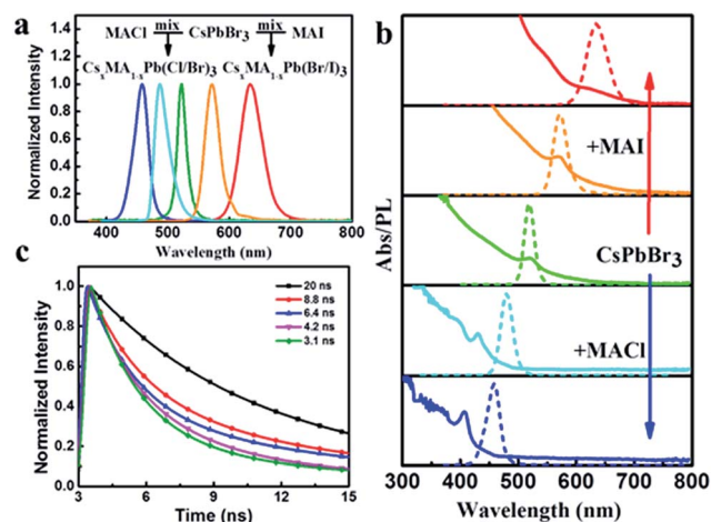
Fig. 5 (a) An overview of the PL spectra of the samples obtained by mixing CsPbBr 3 NCs with either MACl or MAI NCs in various ratios ( \lambda_{\text{ex}} = 365 \text{ nm} for all). (b) Evolution of the optical absorption (solid lines) and PL (dashed lines) spectra of CsPbBr 3 NCs with the increasing quantities of MAX (X = Cl and I), added as ion-exchange sources. (c) Evolution of the time-resolved PL decay spectra of CsPbBr 3 NCs and mixing with either MACl or MAI NCs at various ratios.
