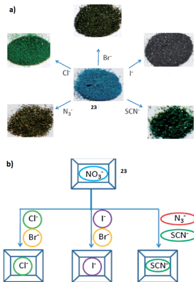
Fig. 8 (a) The color changes of compound [CuL 2 (H 2 O) 0.5 ](NO 3 ) 2 (23) as a result of anion-exchange. (b) The anion selectivity based on the compound. Reproduced with permission from ref. 73, copyright 2011, Royal Society of Chemistry.
