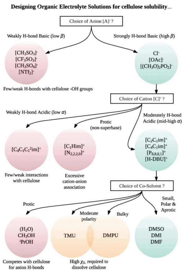
Fig. 5 A flow diagram to aid in the selection of sensible cation–anion–co-solvent combinations for effective cellulose dissolution. The diagram is intended to highlight key structural and electronic factors that influence cellulose solubility, and is not exhaustive. [\text{NTf}_2]^- = bis(trifluoromethanesulfonyl)imide; [\text{OAc}]^- = acetate; [\text{C}_4\text{C}_1\text{C}_1^2\text{im}]^+ = 1-butyl-2,3-dimethylimidazolium; [\text{C}_1\text{Him}]^+ = 1-methylimidazolium; [\text{N}_{2,2,2,0}]^+ = triethylammonium; [\text{C}_2\text{C}_1\text{im}]^+ = 1-ethyl-3-methylimidazolium; [\text{C}_4\text{C}_1\text{im}]^+ = 1-butyl-3-methylimidazolium; [\text{P}_{8,8,8,1}]^+ = tri( n -octyl)methylphosphonium; [\text{H-DBU}]^+ = 1,8-diazabicyclo[5.4.0]undecenium; TMU = 1,1,3,3-tetramethylurea; DMPU = 1,3-dimethyl-3,4,5,6-tetrahydro-2-pyrimidinone; DMI = 1,3-dimethyl-2-imidazolidinone.
