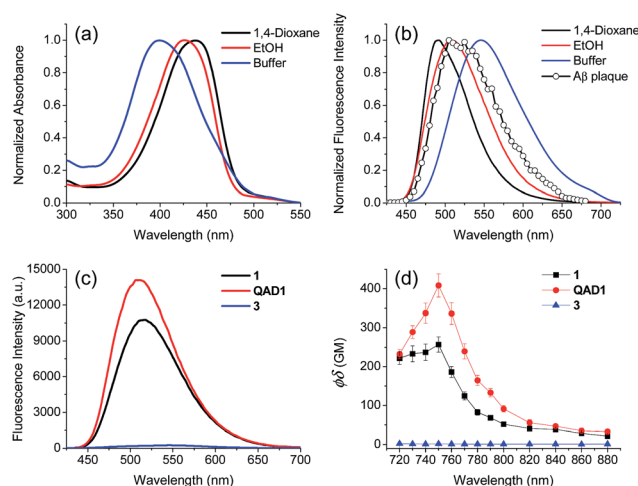
Fig. 1 (a) Normalized absorption and (b) emission spectra of QAD1 (1 \mu\text{M} ) in 1,4-dioxane, EtOH and PBS buffer (10 mM, pH 7.4). Two-photon excited fluorescence (TPEF) spectra (O) acquired from A \beta plaques in a QAD1 -labeled brain slice. (c) Emission spectra of 1 , QAD1 and 3 (1 \mu\text{M} ) acquired in EtOH. (d) Two-photon action spectra of 1 , QAD1 and 3 (1 \mu\text{M} ) acquired in EtOH.
