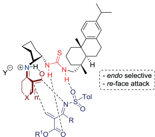
Fig. 5 Proposed activation model for the re -face attack.
