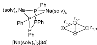
Fig. 5 Schematic view of the tetraphosphane-1,4-diide [\text{Na}(\text{solvent})_x]_2[\text{34}] showing the characteristic bicyclobutane-shaped \text{M}_2\text{P}_2 arrangement (left); illustration of point charges and coulombic interactions (right).
