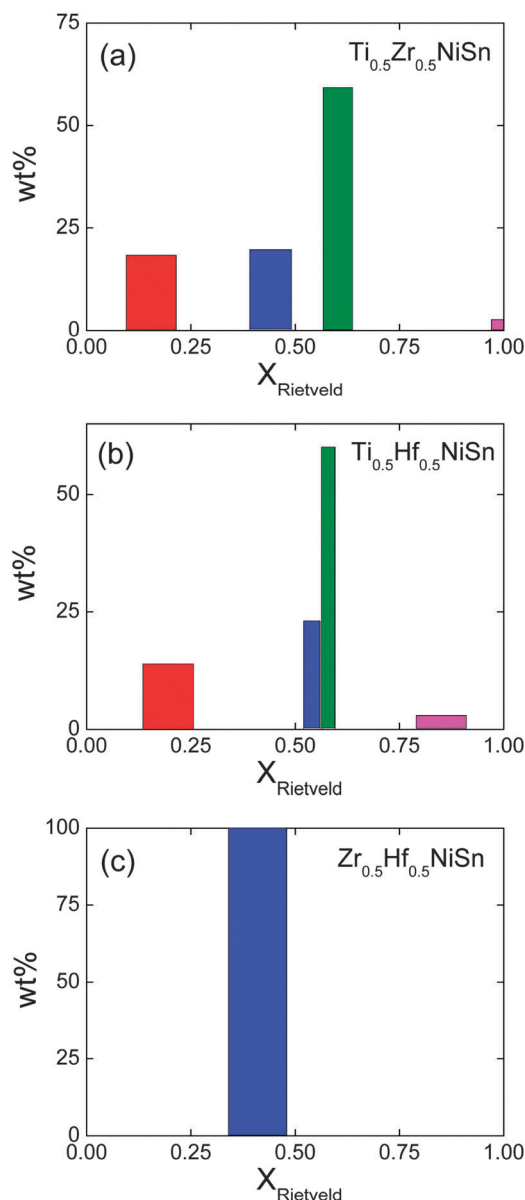
Fig. 3 Histograms of the phase distribution and compositional spread of the \text{X}_{1-x}\text{X}'_{0.5}\text{NiSn} phases present in the \text{X}_{0.5}\text{X}'_{0.5}\text{NiSn} samples (X = Ti, Zr, Hf). The centre and widths of the bars correspond to x_R and \Delta x .
