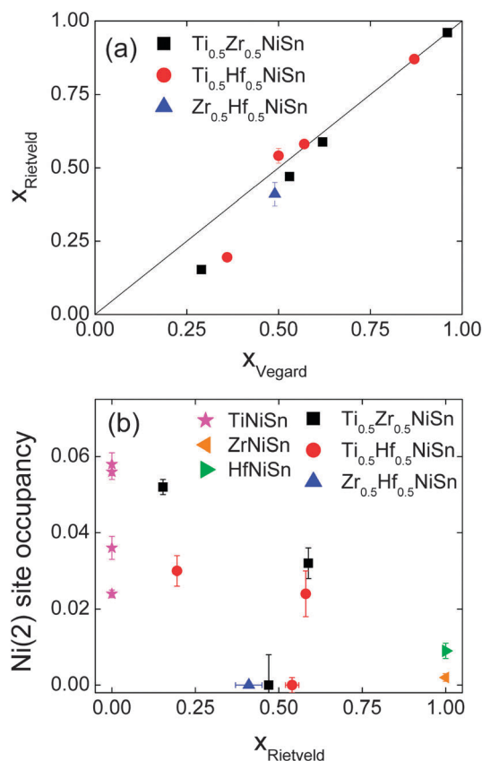
Fig. 2 (a) Fitted X-metal fractions ( x_R ) against those calculated from Vegard's law ( x_V ). (b) Ni(2) site occupancy for the \text{X}_{1-x}\text{X}'_{0.5}\text{Ni}_{1+y}\text{Sn} phases present in the \text{X}_{0.5}\text{X}'_{0.5}\text{NiSn} samples (X, X' = Ti, Zr, Hf). Additional TiNiSn data from ref. 7.
