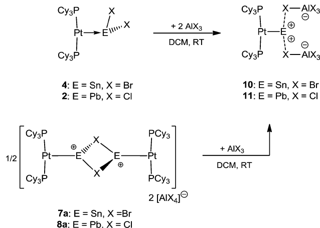
Scheme 4 Formation of the pseudo-monocoordinate dicationic species of tin ( 10 ) and lead ( 11 ).
