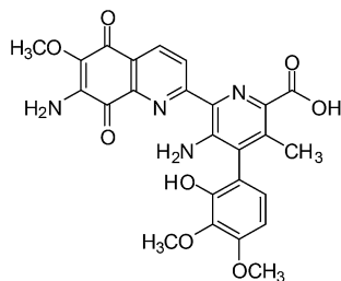
Streptonigrin
