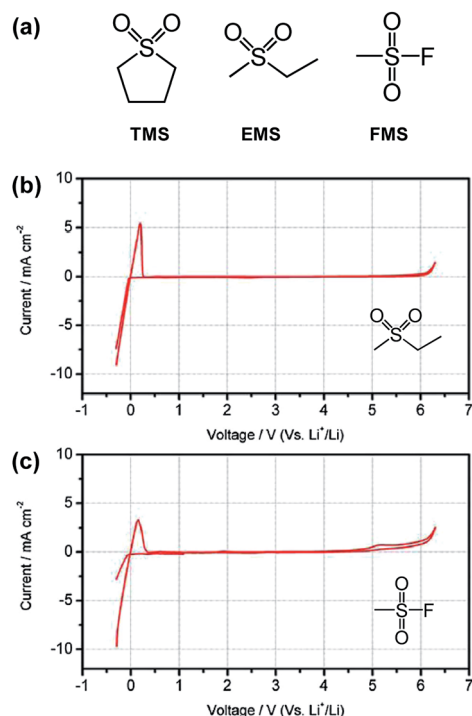
Fig. 14 (a) Structures of typical sulfone solvents. Cyclic voltammograms of 1 M \text{LiPF}_6 in (b) EMS/DMC (1 : 1 by wt) and (c) EMS/FMS (1 : 1 by wt). Scan rate: 5 mV \text{s}^{-1} . Pt as the working and counter electrodes and Li as the reference electrode. Reproduced with permission. 78
