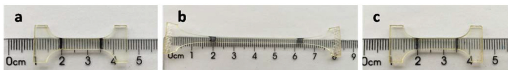
Fig. 9 Demonstration of the high strain shape memory performance for Epon1.
