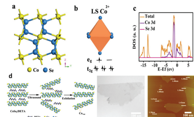
Fig. 11 (a) Crystal structure of \text{CoSe}_2 in the cubic pyrite-type phase; (b) schematic spin structure of the \text{Co}^{2+} cation; (c) DOS diagram for \text{CoSe}_2 ; (d) schematic of the formation of V''_{\text{Co}} vacancies in \text{CoSe}_2 ultrathin nanosheets (left), TEM image (middle) and AFM image (right) of the ultrathin \text{CoSe}_2 nanosheet (reproduced with permission from ref. 43. Copyright 2014 American Chemical Society).
